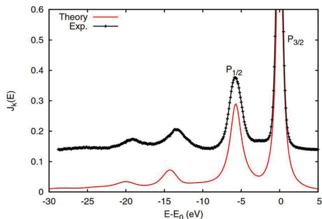
Fig. 9 2p core-level XPS of rutile \text{TiO}_2 calculated with the real-time cumulant approach (red solid) compared to experimental results (black). The main quasiparticle peaks are labeled P_{1/2} and P_{3/2} , while the charge transfer satellites appear at \sim 14 eV lower energy. Reprinted figure with permission from [J. J. Kas, F. D. Vila, J. J. Rehr and S. A. Chambers, Phys. Rev. B , 2015, 91 , 121112], Copyright (2022) by the American Physical Society.
